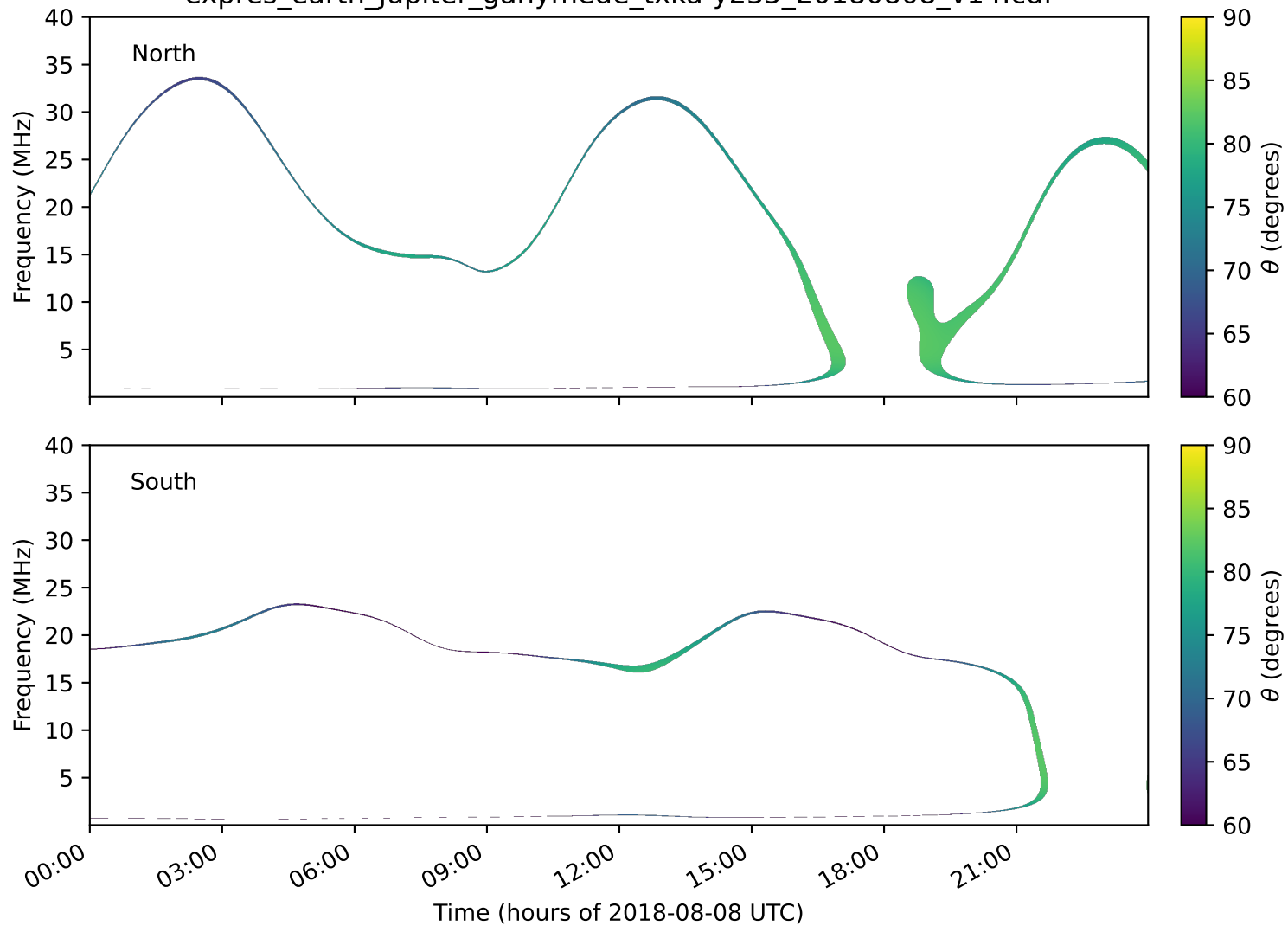
expres_earth_jupiter_ganymede_txka-y235_20180808_v14.cdf
