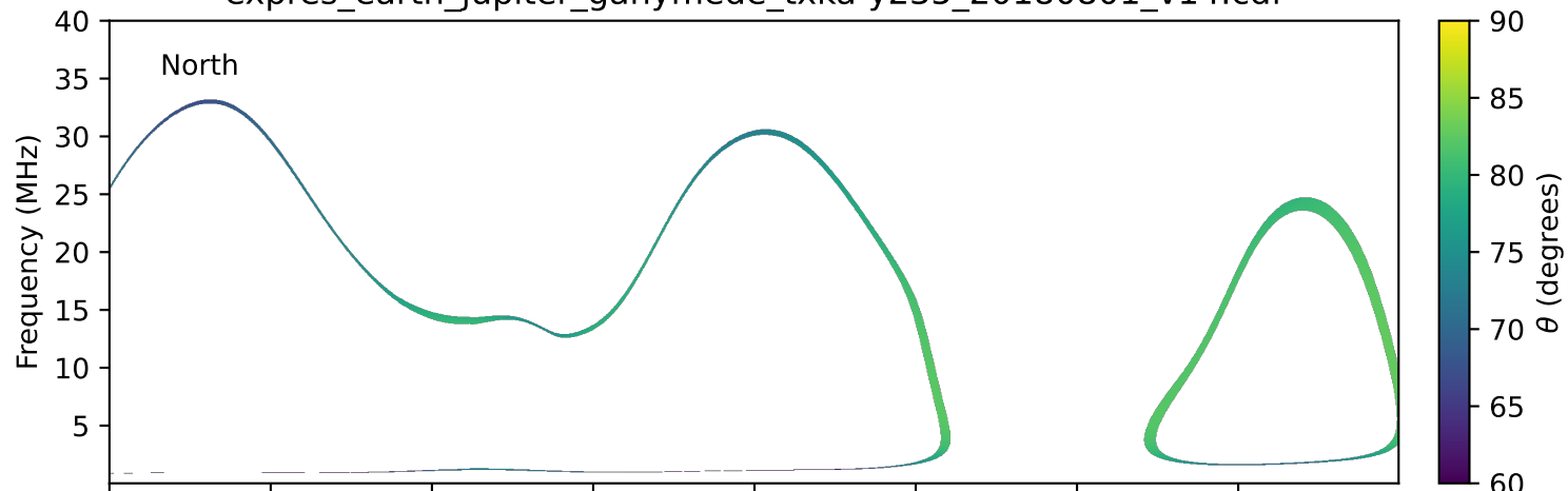
expres_earth_jupiter_ganymede_txka-y235_20180801_v14.cdf
