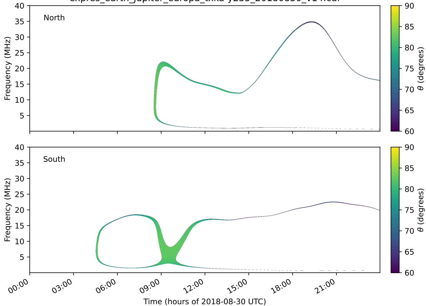
expres_earth_jupiter_europa_txka-y235_20180830_v14.cdf
