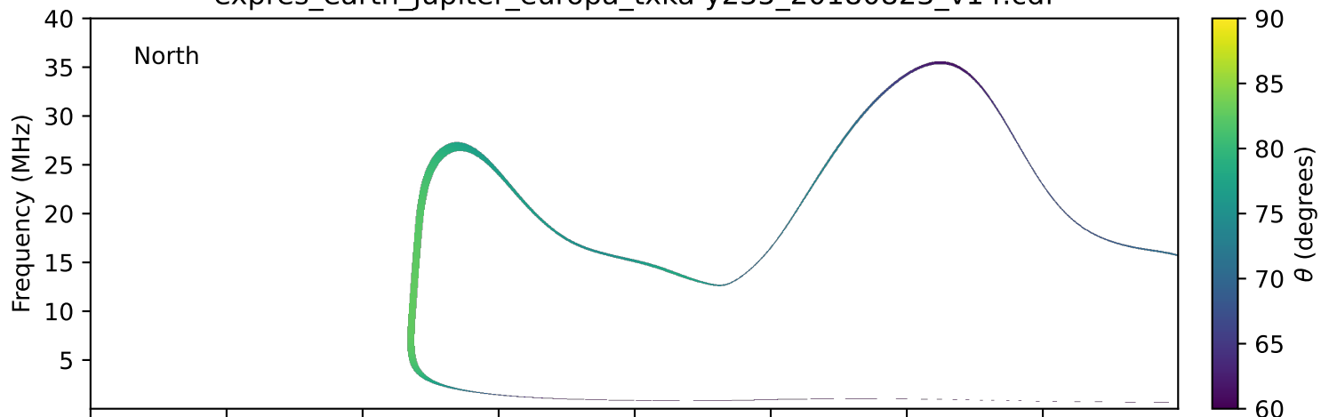
expres_earth_jupiter_europa_txka-y235_20180823_v14.cdf
