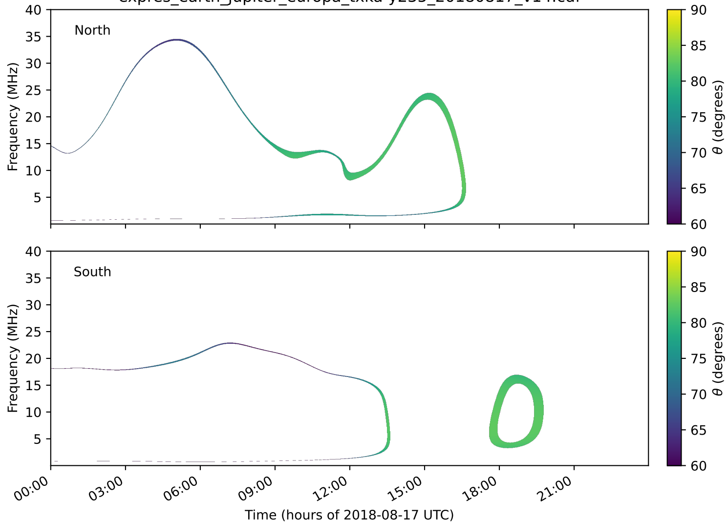
expres_earth_jupiter_europa_txka-y235_20180817_v14.cdf
