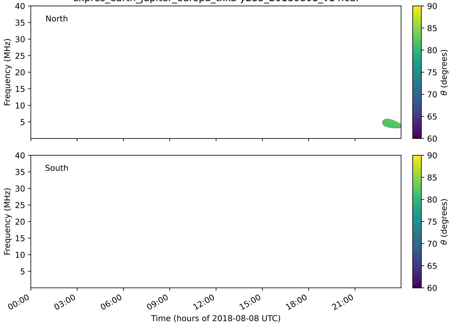
expres_earth_jupiter_europa_txka-y235_20180808_v14.cdf
