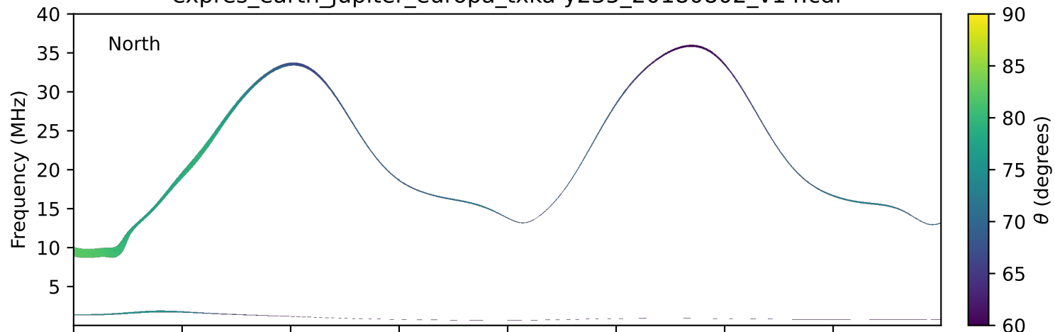
expres_earth_jupiter_europa_txka-y235_20180802_v14.cdf
