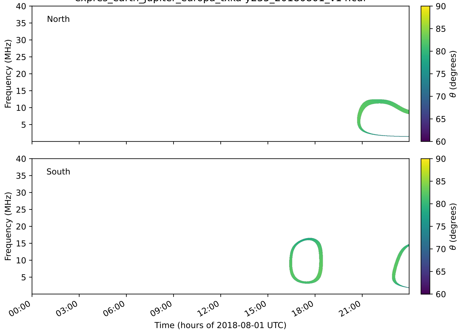
expres_earth_jupiter_europa_txka-y235_20180801_v14.cdf
