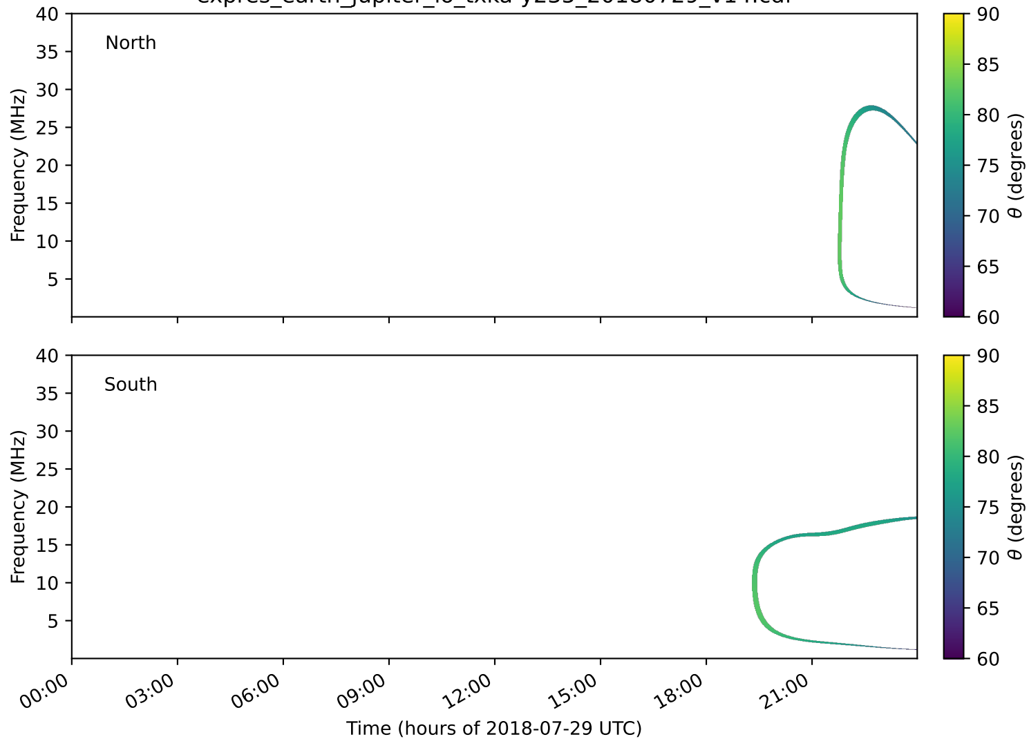
expres_earth_jupiter_io_txka-y235_20180729_v14.cdf
