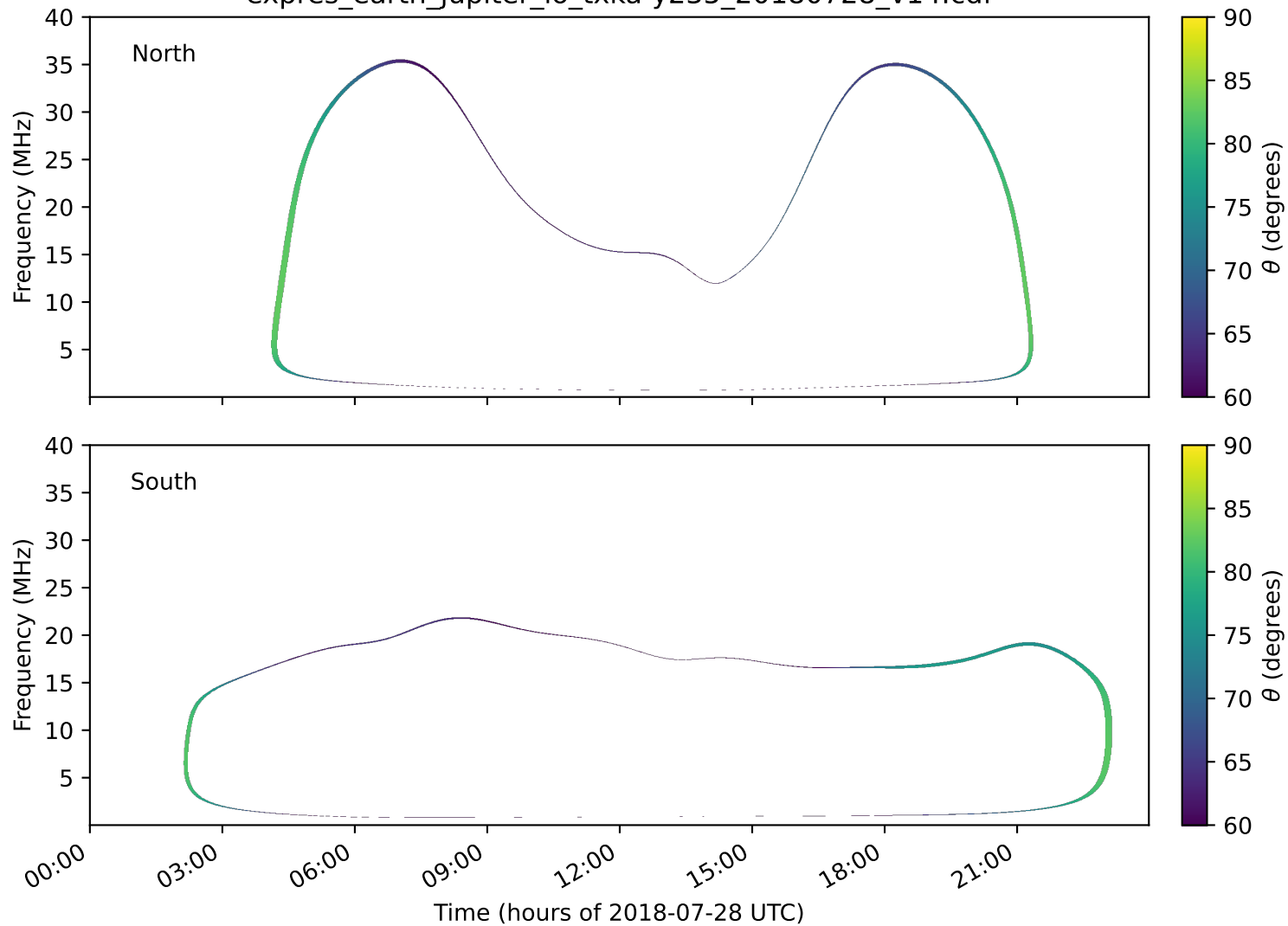
expres_earth_jupiter_io_txka-y235_20180728_v14.cdf
