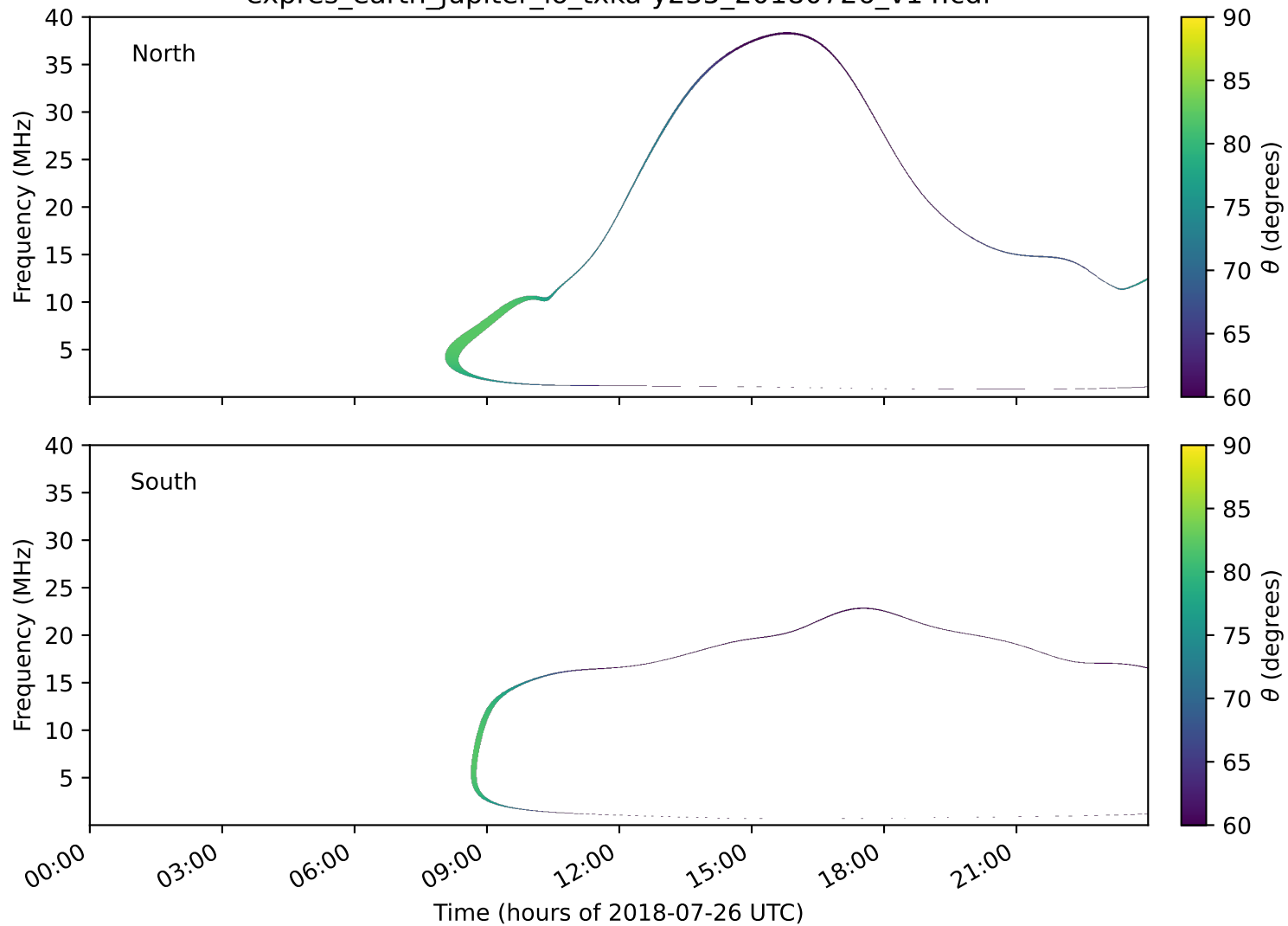
expres_earth_jupiter_io_txka-y235_20180726_v14.cdf
