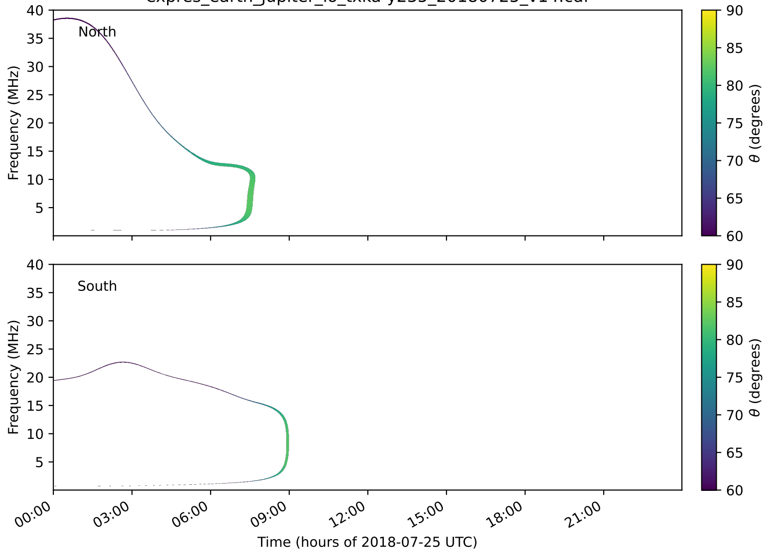
expres_earth_jupiter_io_txka-y235_20180725_v14.cdf
