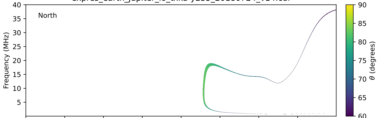
expres_earth_jupiter_io_txka-y235_20180724_v14.cdf
