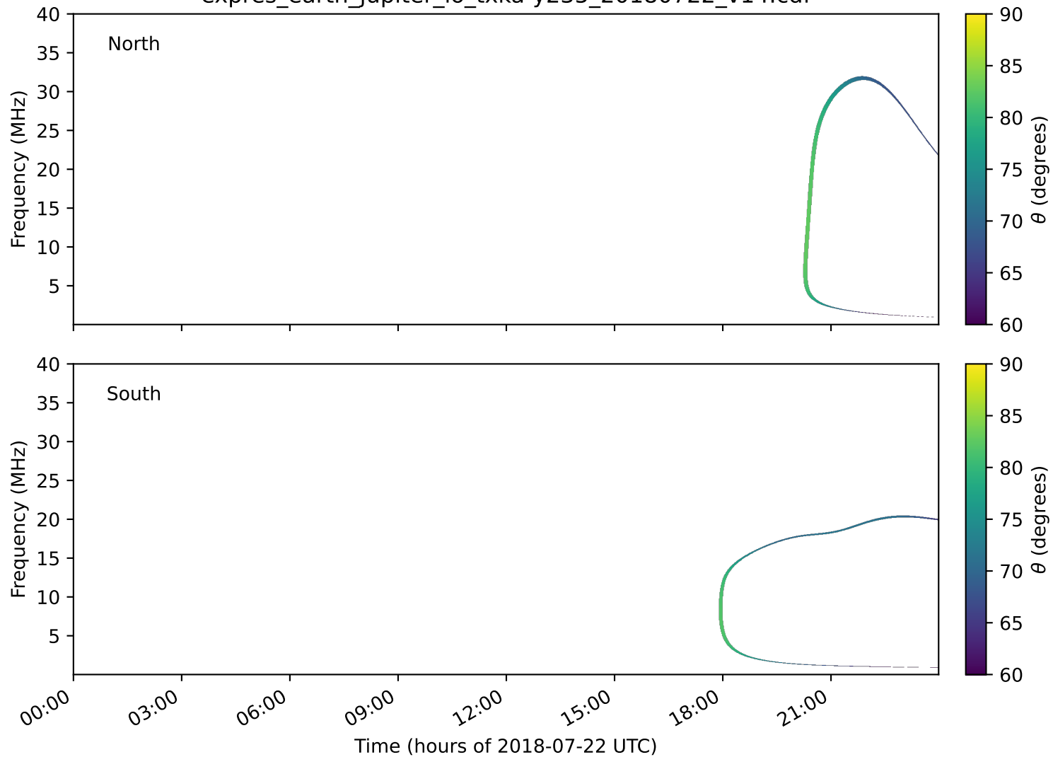
expres_earth_jupiter_io_txka-y235_20180722_v14.cdf
