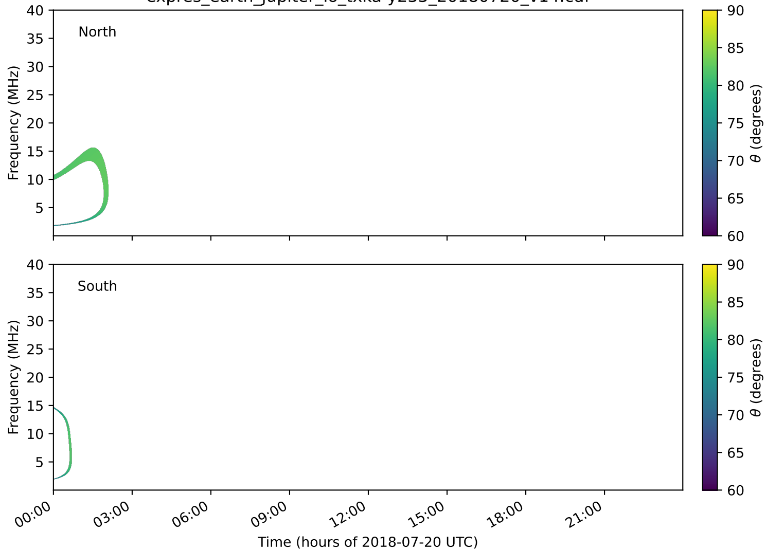
expres_earth_jupiter_io_txka-y235_20180720_v14.cdf
