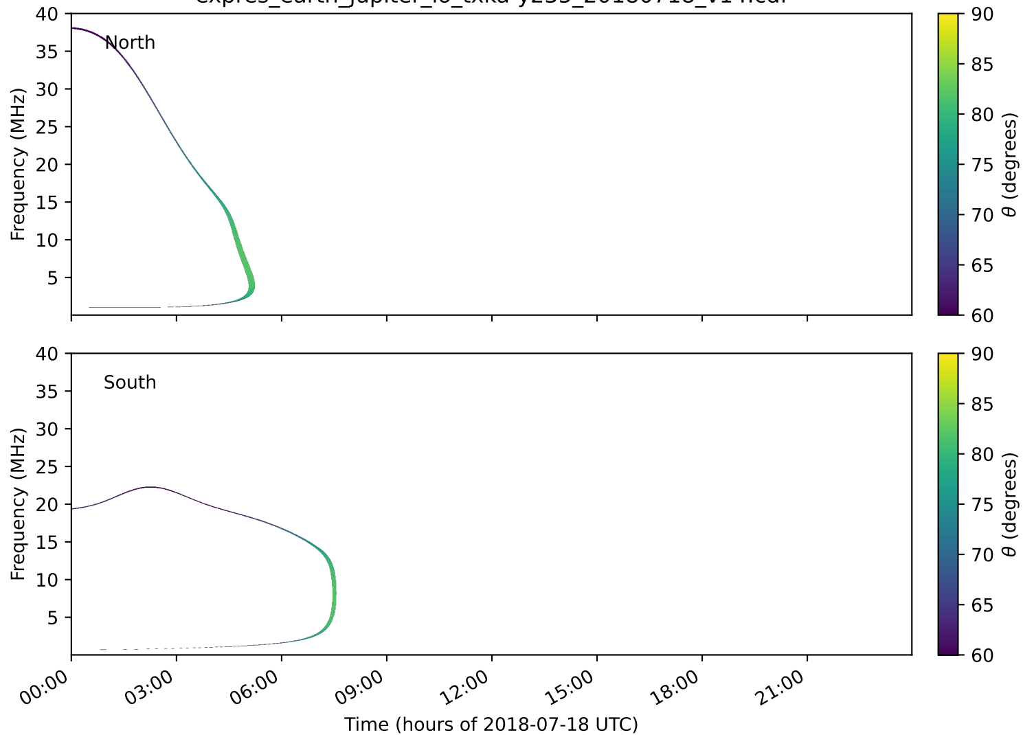
expres_earth_jupiter_io_txka-y235_20180718_v14.cdf
