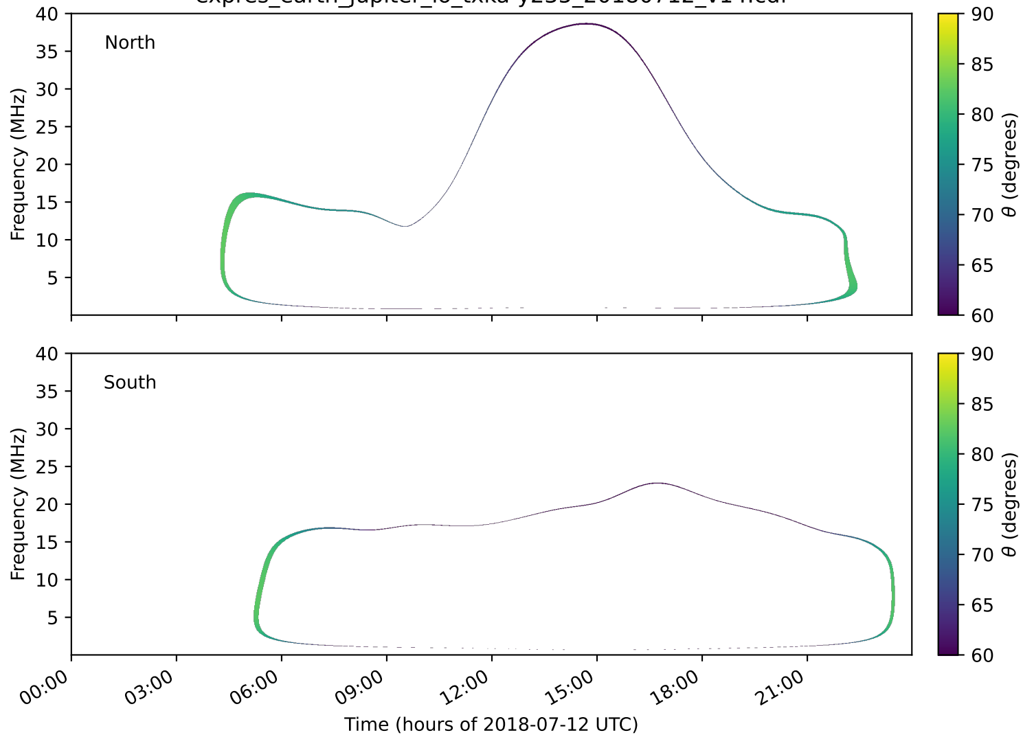
expres_earth_jupiter_io_txka-y235_20180712_v14.cdf
