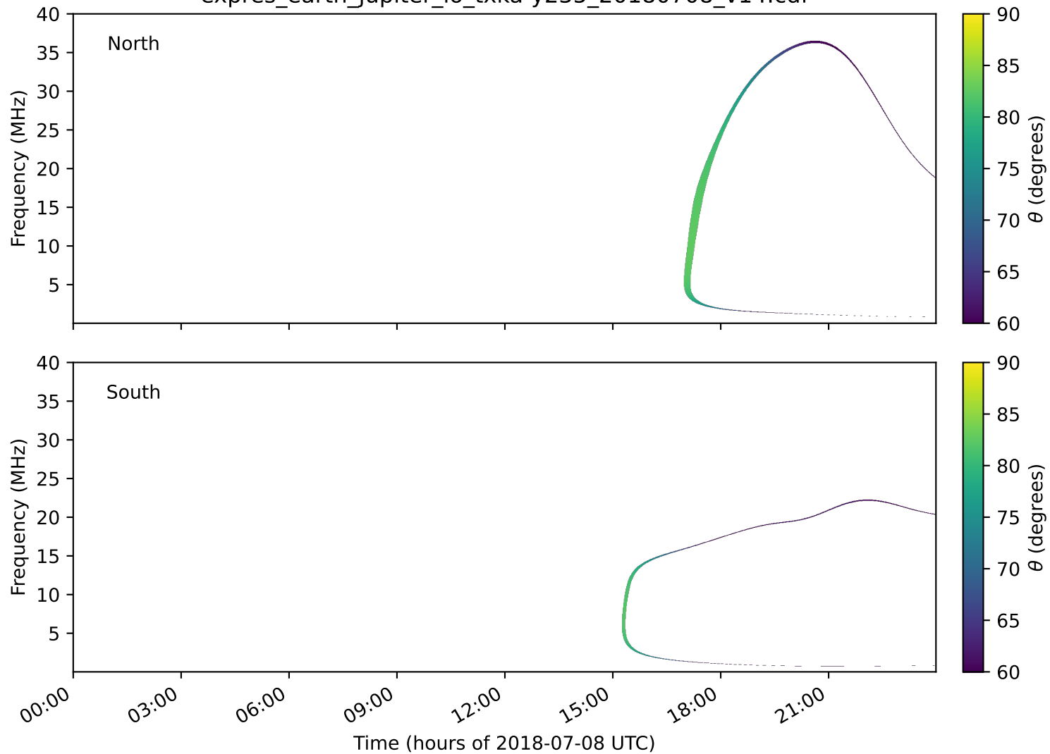
expres_earth_jupiter_io_txka-y235_20180708_v14.cdf
