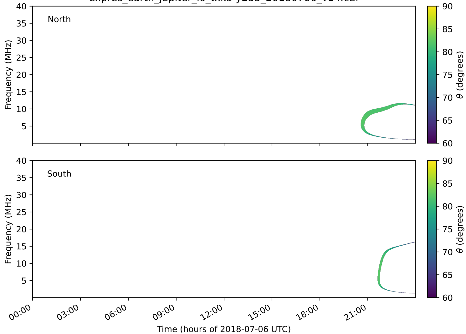
expres_earth_jupiter_io_txka-y235_20180706_v14.cdf
