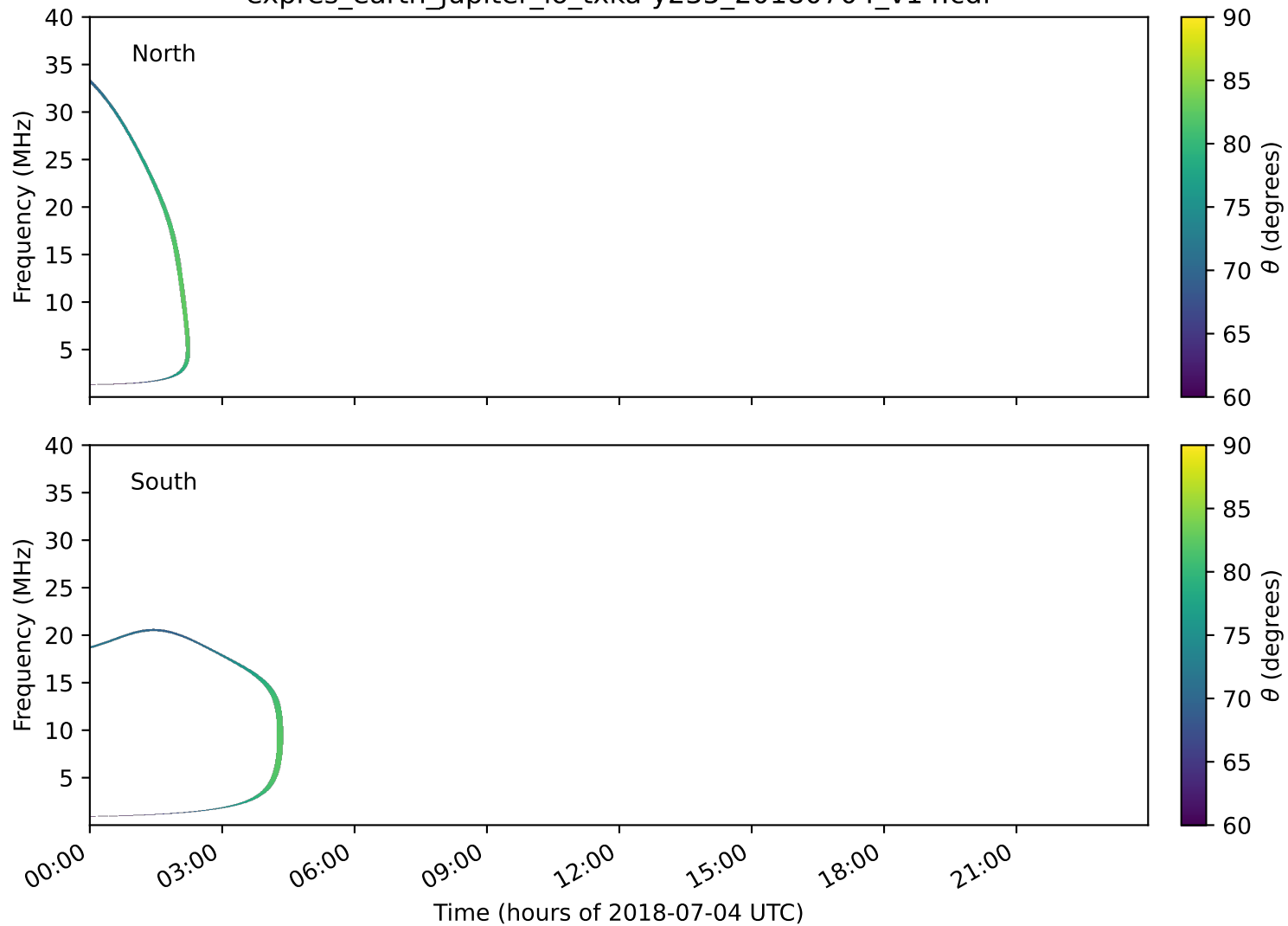
expres_earth_jupiter_io_txka-y235_20180704_v14.cdf
