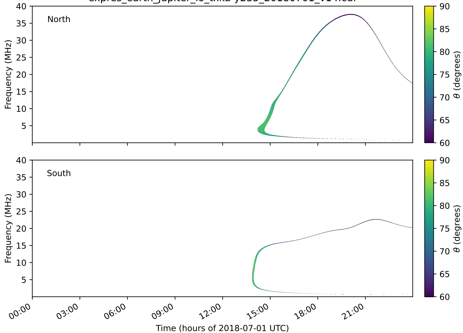
expres_earth_jupiter_io_txka-y235_20180701_v14.cdf
