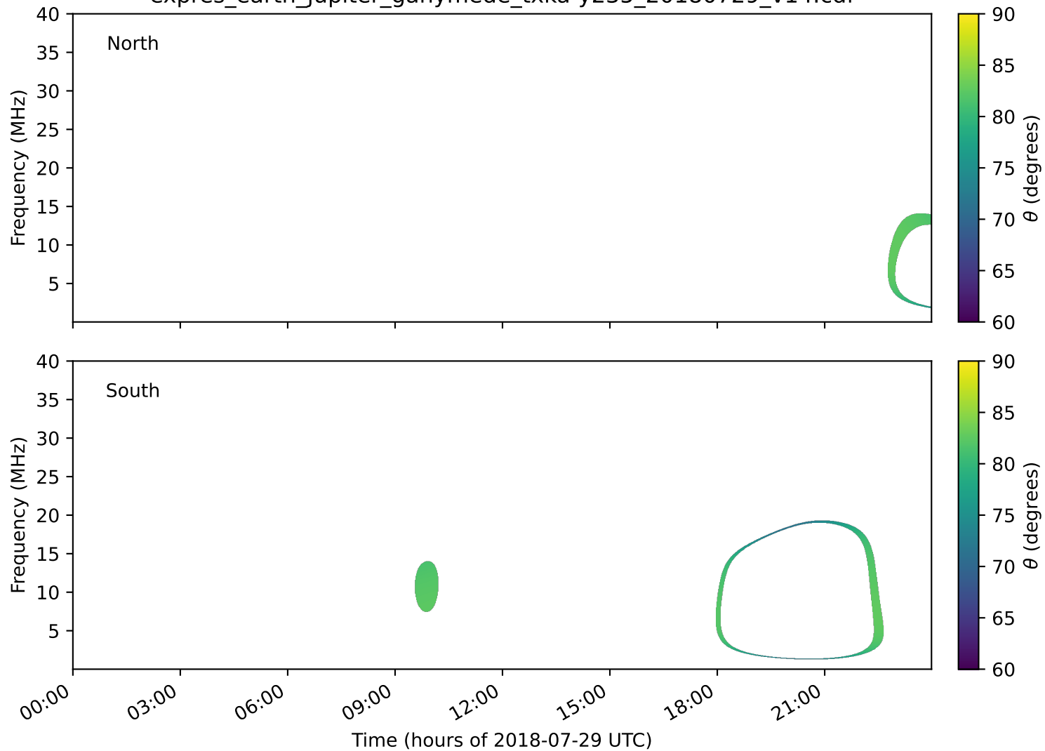
expres_earth_jupiter_ganymede_txka-y235_20180729_v14.cdf
