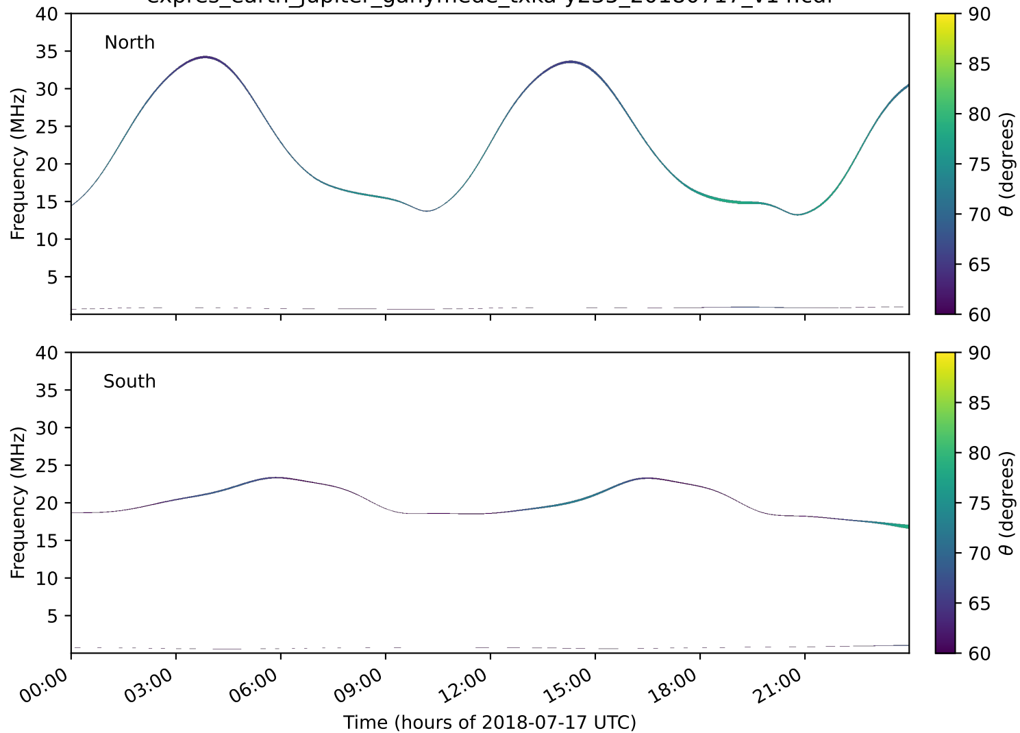
expres_earth_jupiter_ganymede_txka-y235_20180717_v14.cdf
