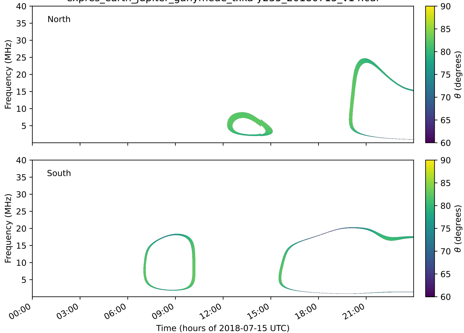
expres_earth_jupiter_ganymede_txka-y235_20180715_v14.cdf
