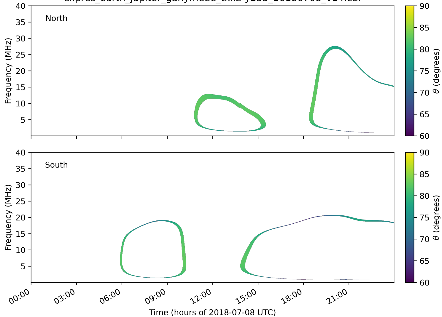
expres_earth_jupiter_ganymede_txka-y235_20180708_v14.cdf
