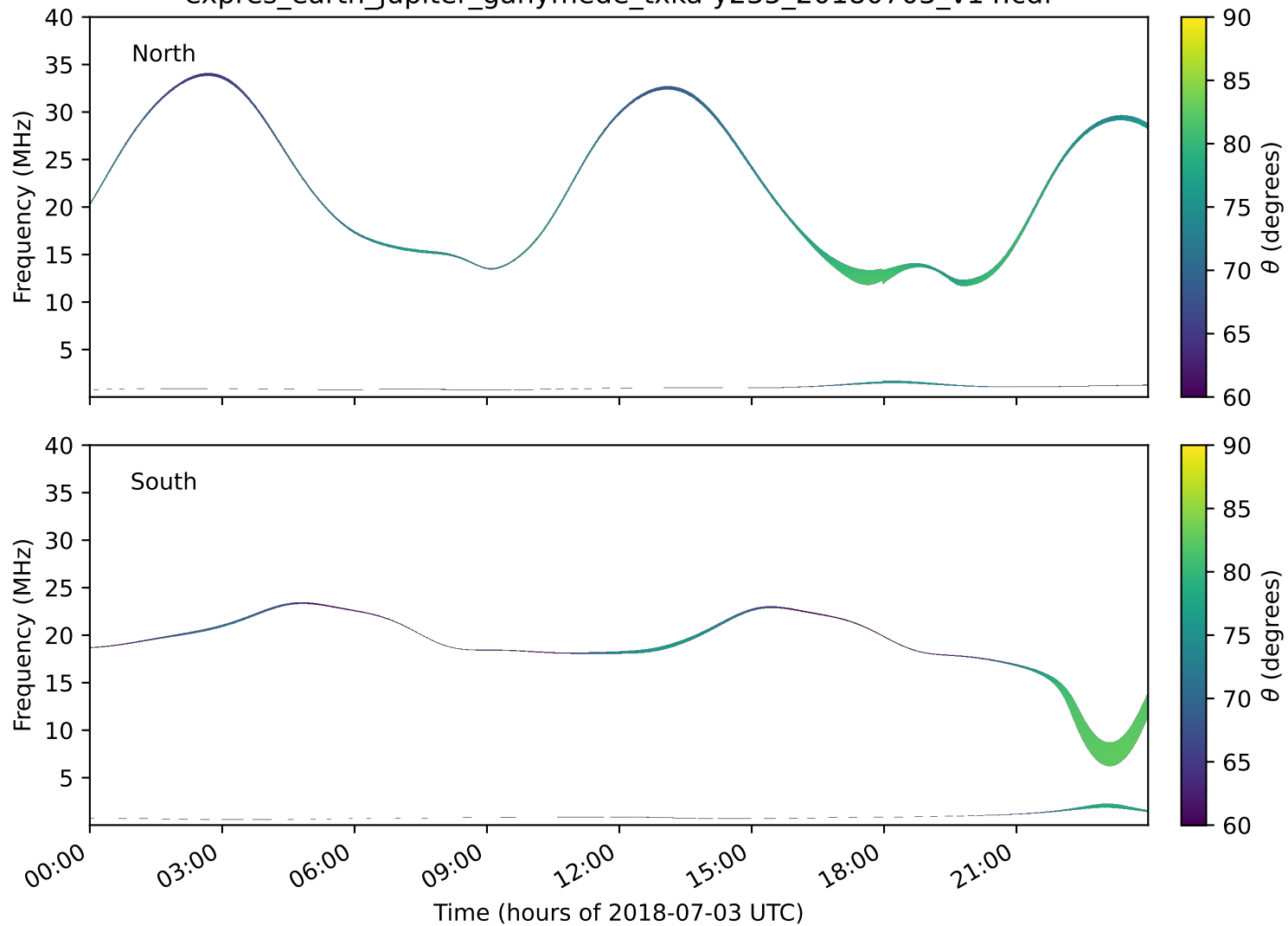
expres_earth_jupiter_ganymede_txka-y235_20180703_v14.cdf
