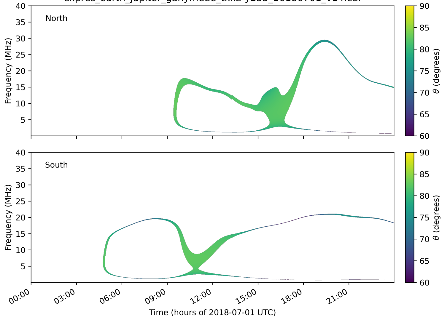
expres_earth_jupiter_ganymede_txka-y235_20180701_v14.cdf
