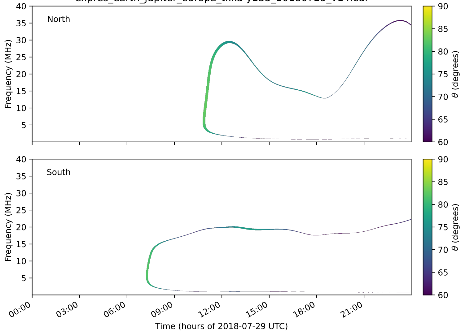
expres_earth_jupiter_europa_txka-y235_20180729_v14.cdf
