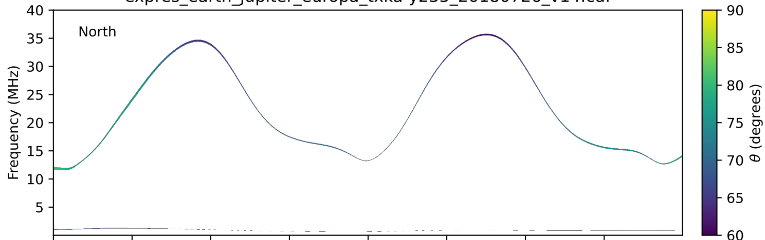
expres_earth_jupiter_europa_txka-y235_20180726_v14.cdf
