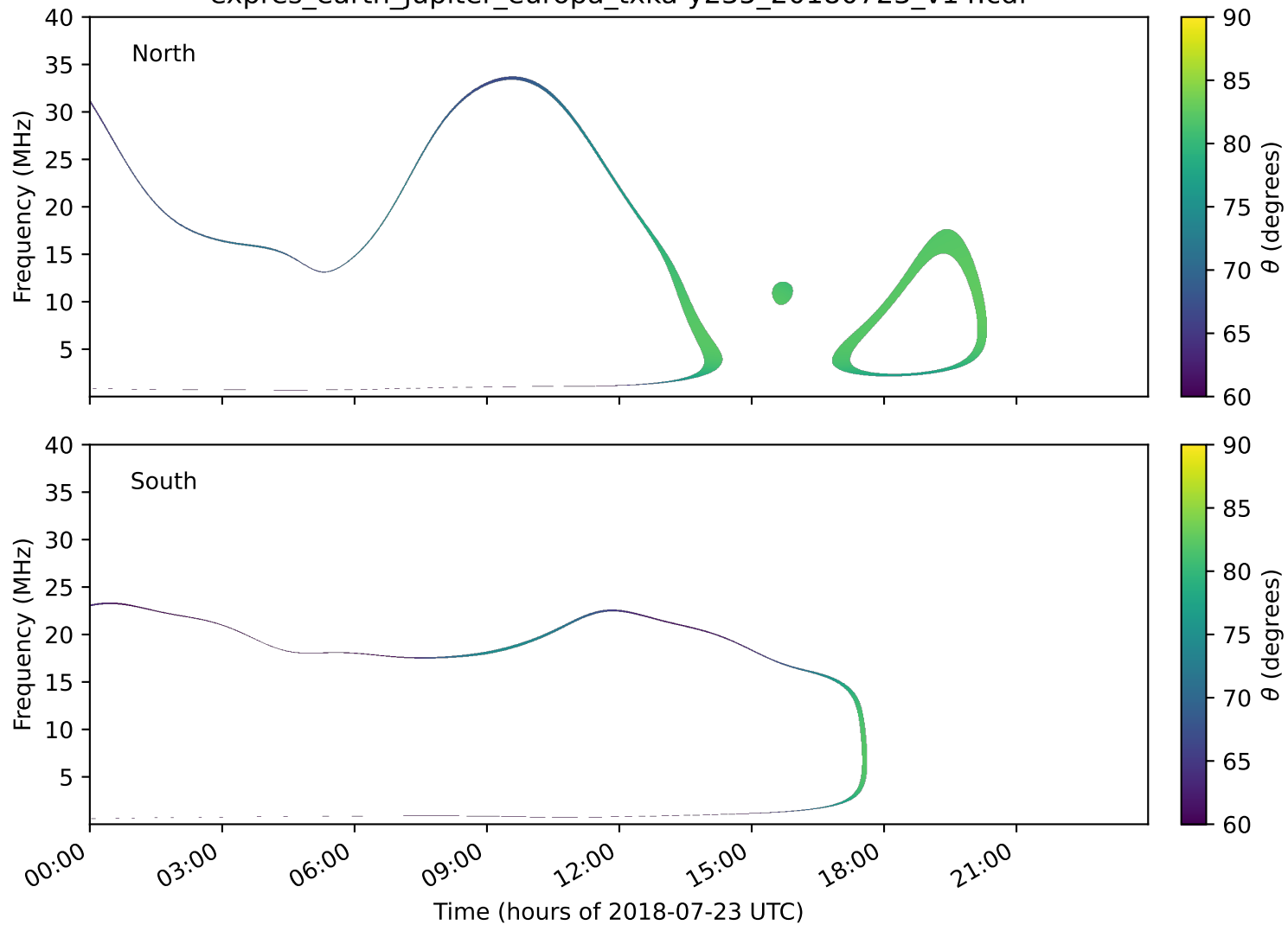
expres_earth_jupiter_europa_txka-y235_20180723_v14.cdf
