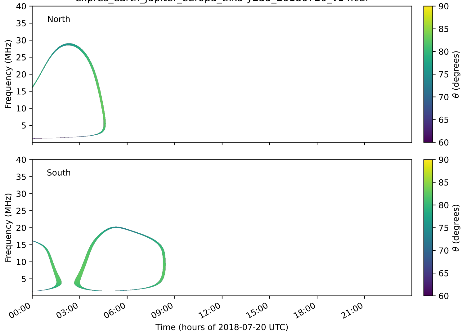
expres_earth_jupiter_europa_txka-y235_20180720_v14.cdf
