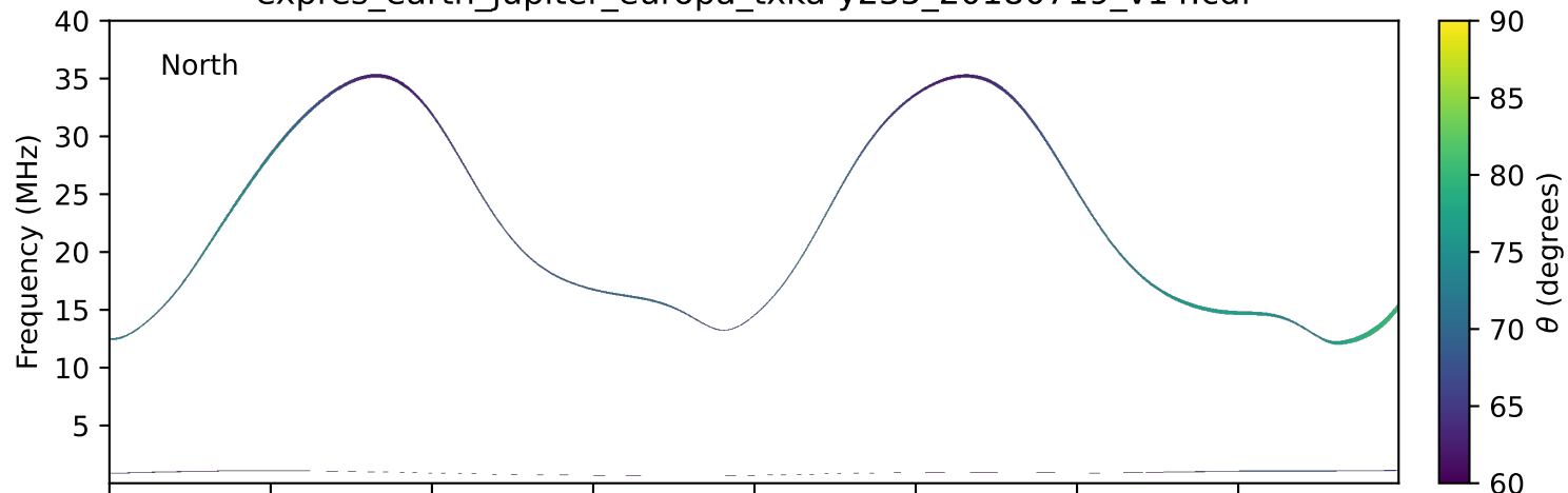
expres_earth_jupiter_europa_txka-y235_20180719_v14.cdf
