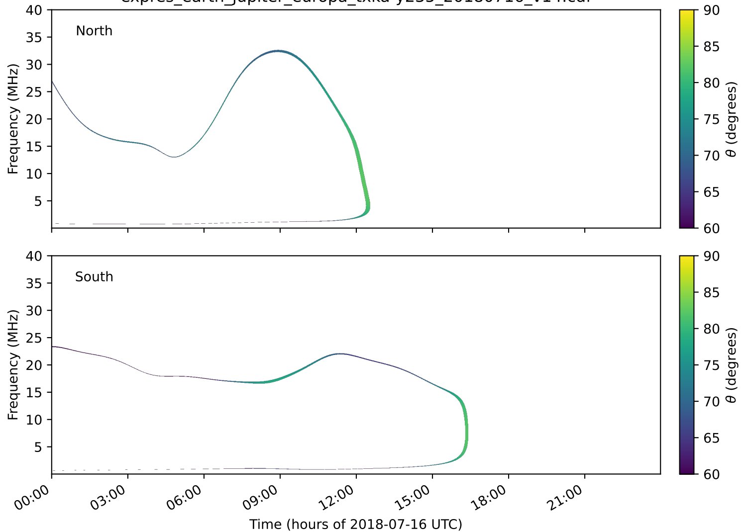
expres_earth_jupiter_europa_txka-y235_20180716_v14.cdf
