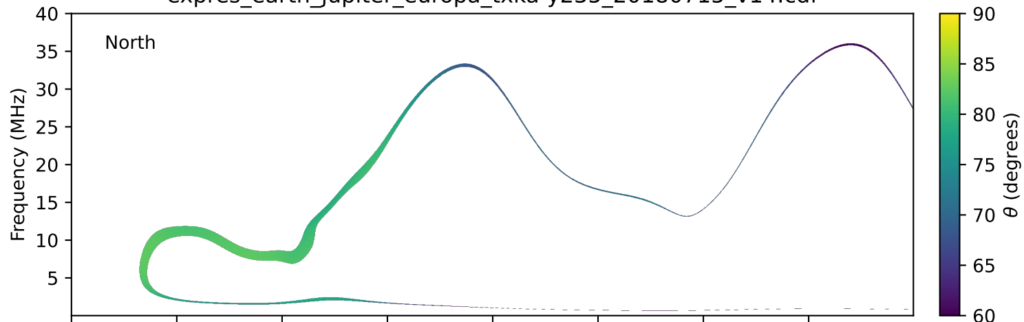
expres_earth_jupiter_europa_txka-y235_20180715_v14.cdf
