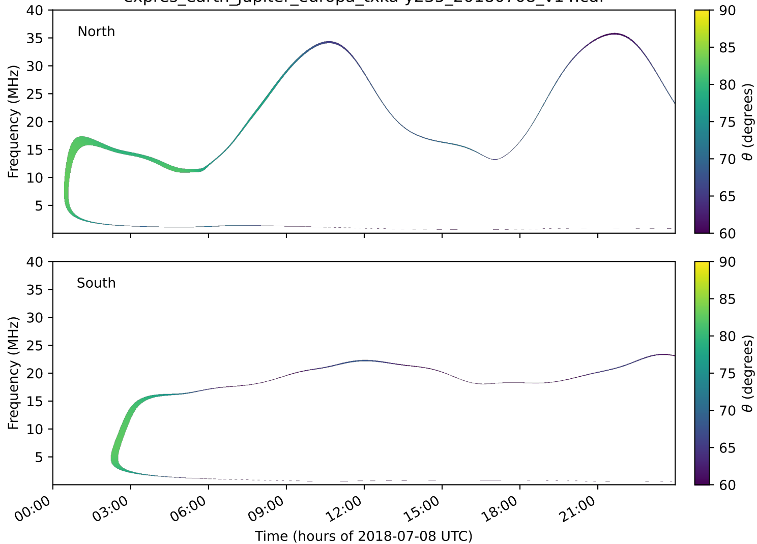
expres_earth_jupiter_europa_txka-y235_20180708_v14.cdf
