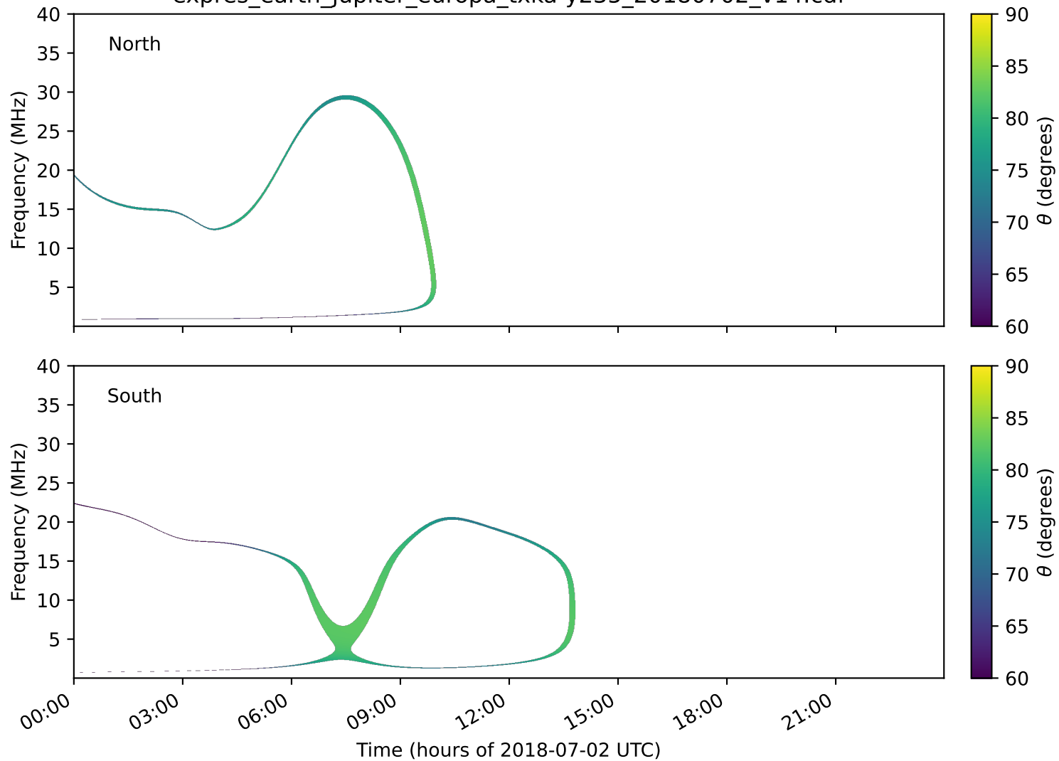
expres_earth_jupiter_europa_txka-y235_20180702_v14.cdf
