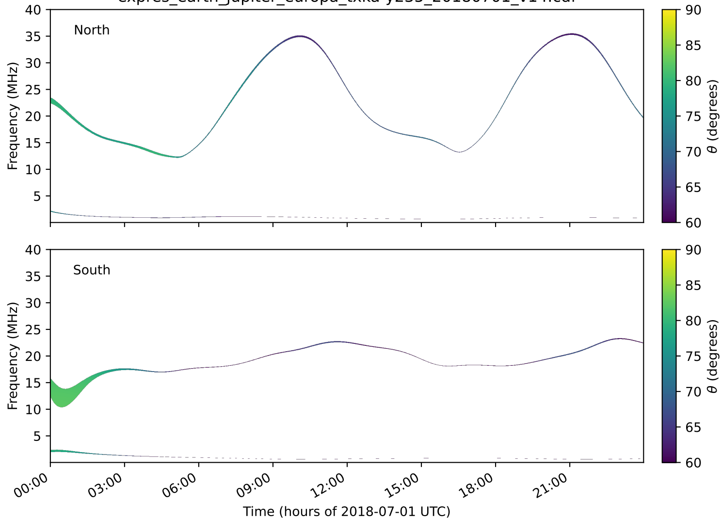
expres_earth_jupiter_europa_txka-y235_20180701_v14.cdf
