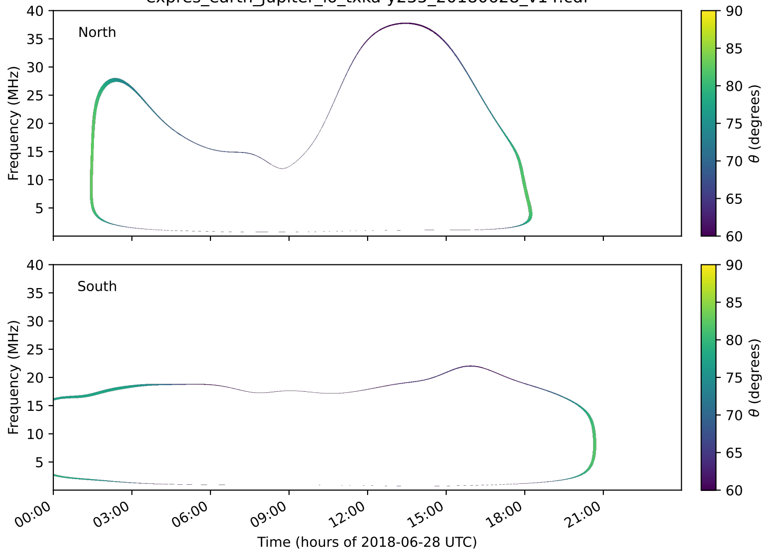
expres_earth_jupiter_io_txka-y235_20180628_v14.cdf
