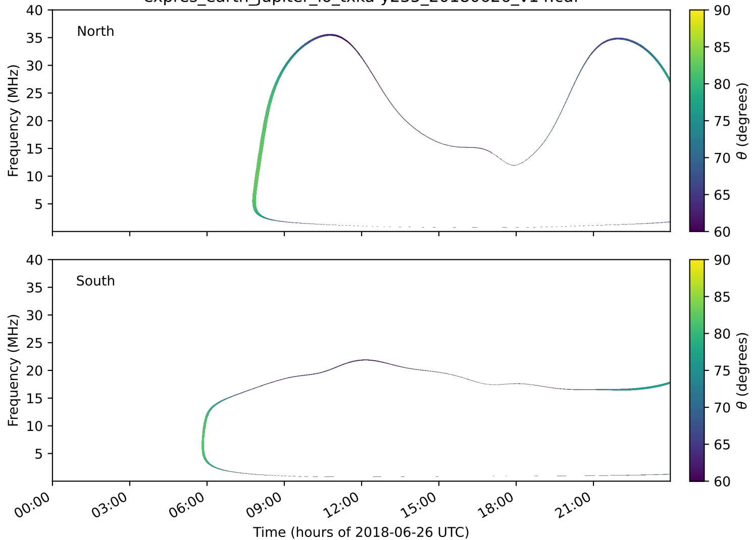
expres_earth_jupiter_io_txka-y235_20180626_v14.cdf
