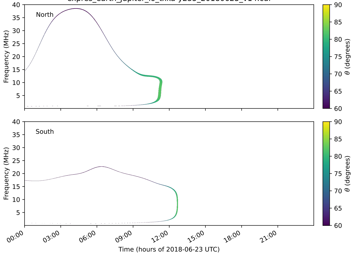
expres_earth_jupiter_io_txka-y235_20180623_v14.cdf
