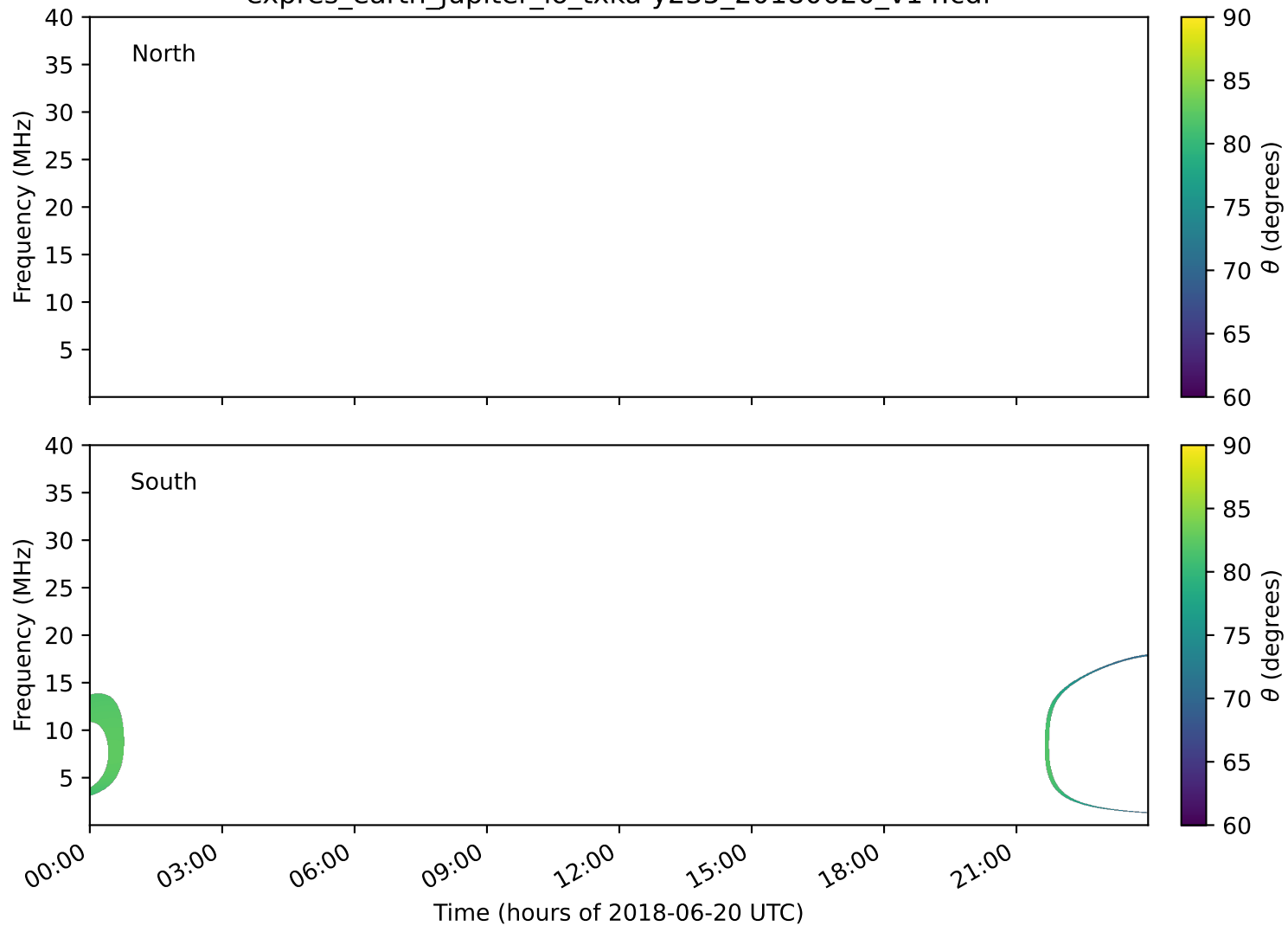
expres_earth_jupiter_io_txka-y235_20180620_v14.cdf
