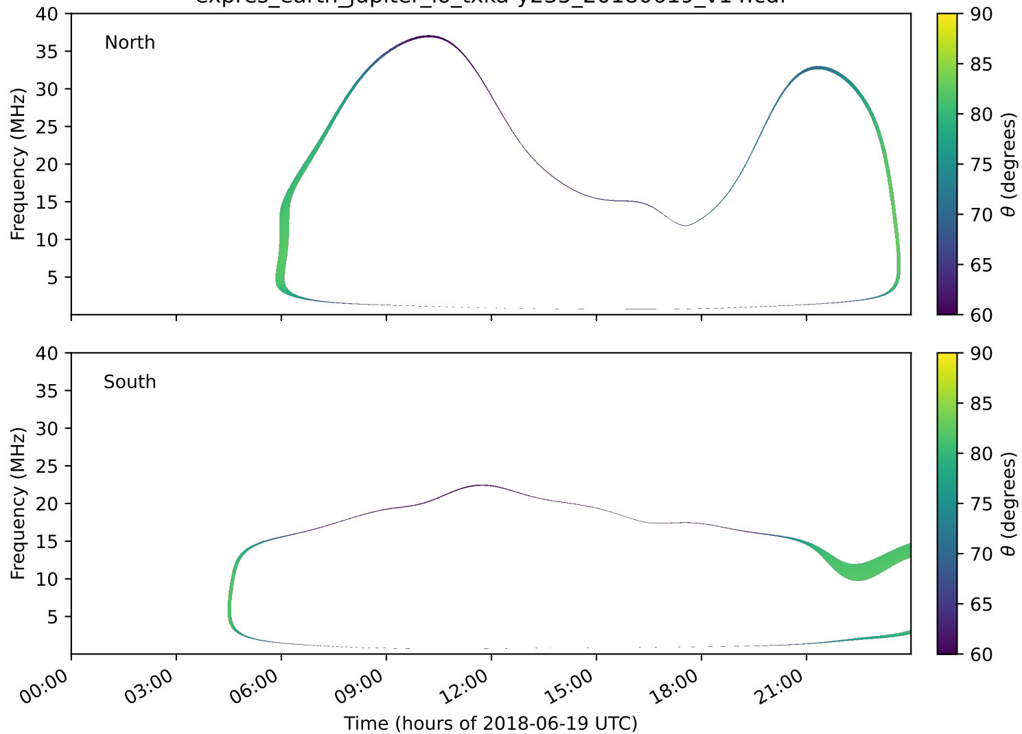
expres_earth_jupiter_io_txka-y235_20180619_v14.cdf
