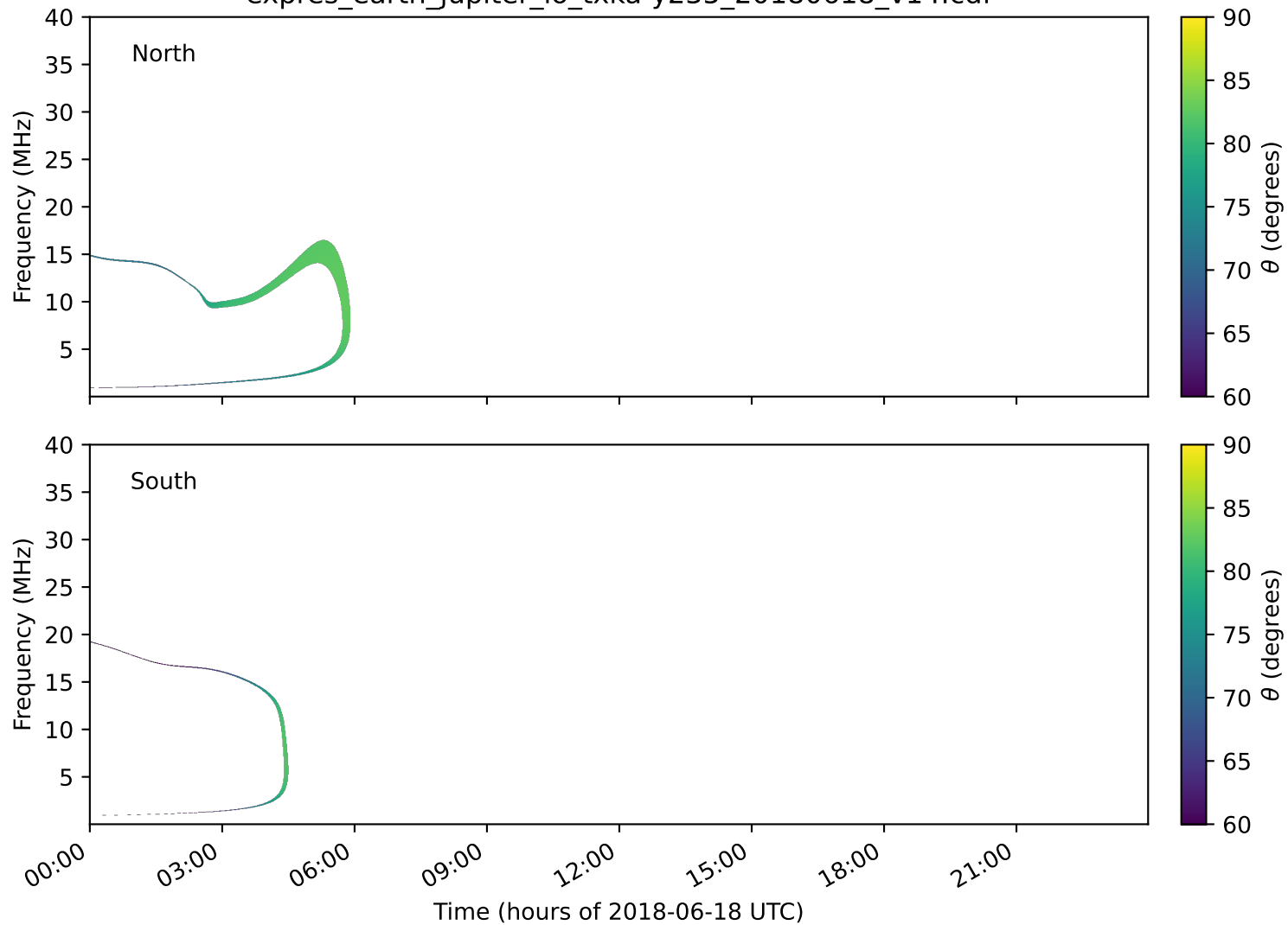
expres_earth_jupiter_io_txka-y235_20180618_v14.cdf
