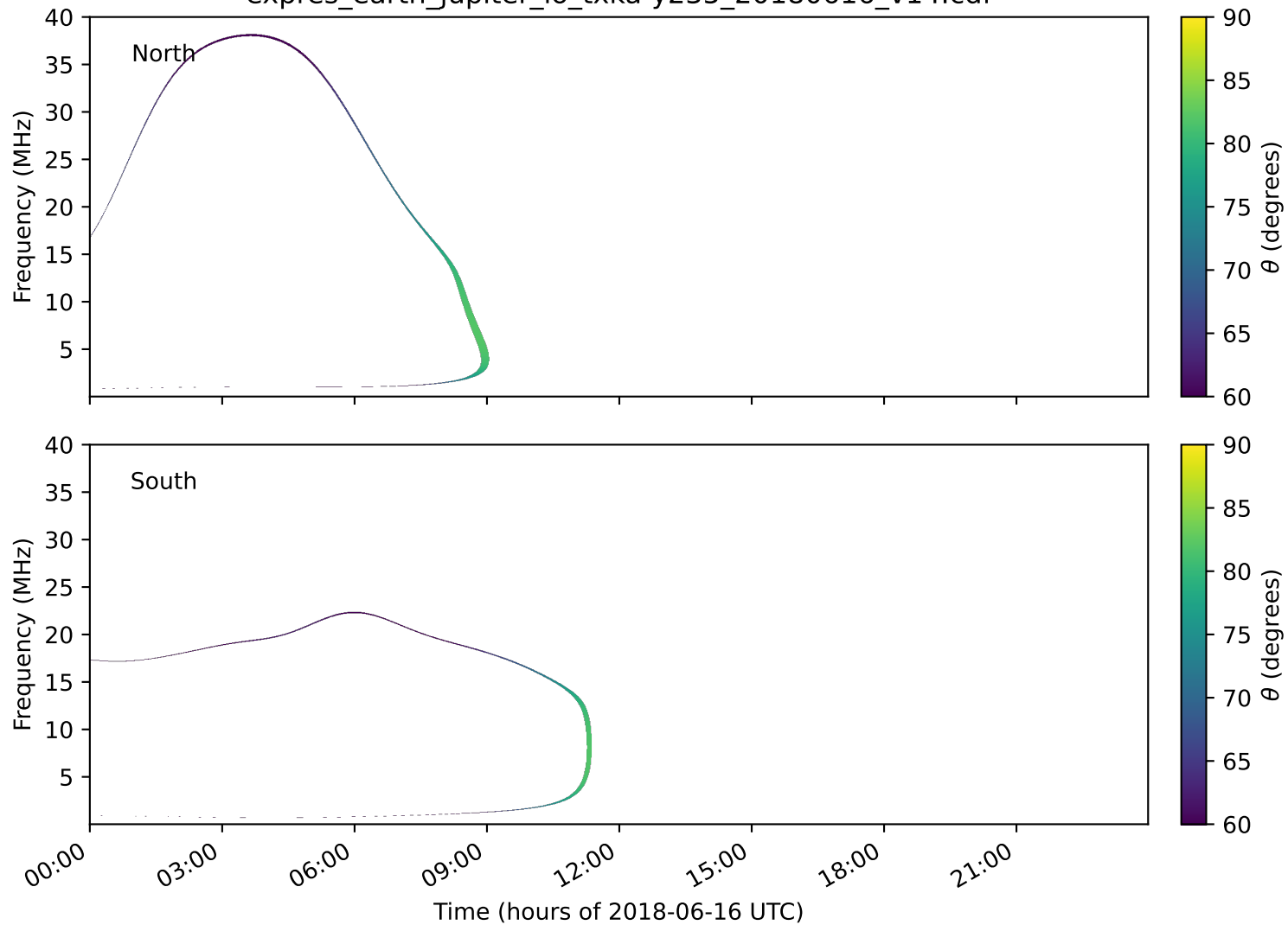
expres_earth_jupiter_io_txka-y235_20180616_v14.cdf
