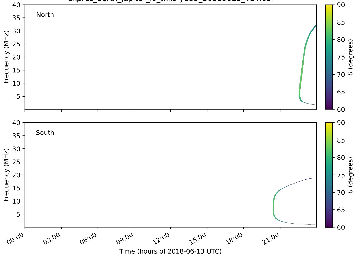
expres_earth_jupiter_io_txka-y235_20180613_v14.cdf
