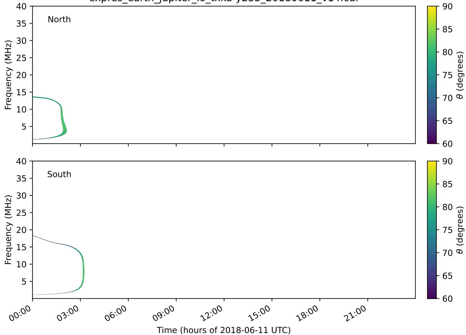
expres_earth_jupiter_io_txka-y235_20180611_v14.cdf
