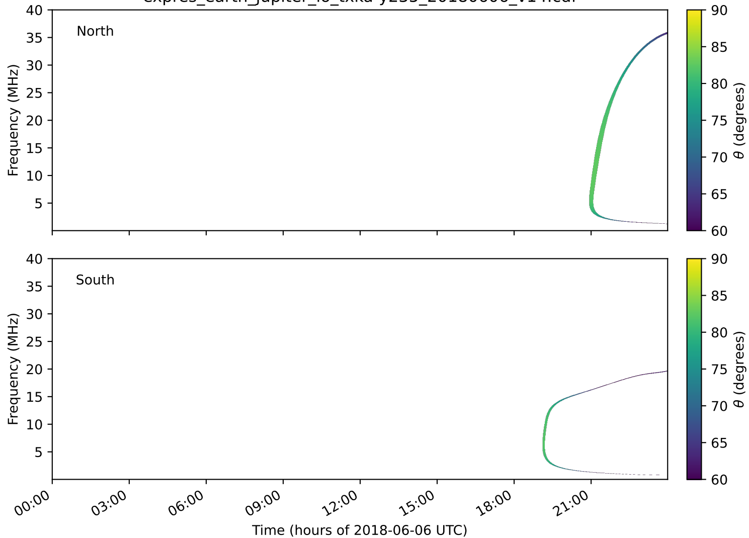
expres_earth_jupiter_io_txka-y235_20180606_v14.cdf
