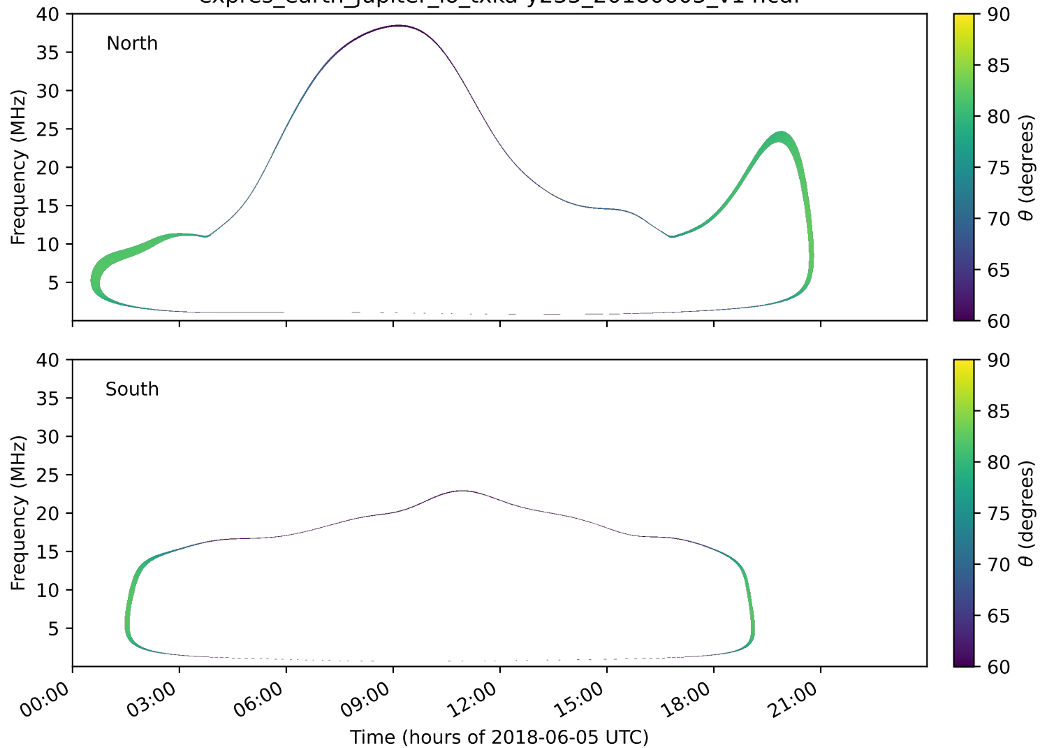
expres_earth_jupiter_io_txka-y235_20180605_v14.cdf
