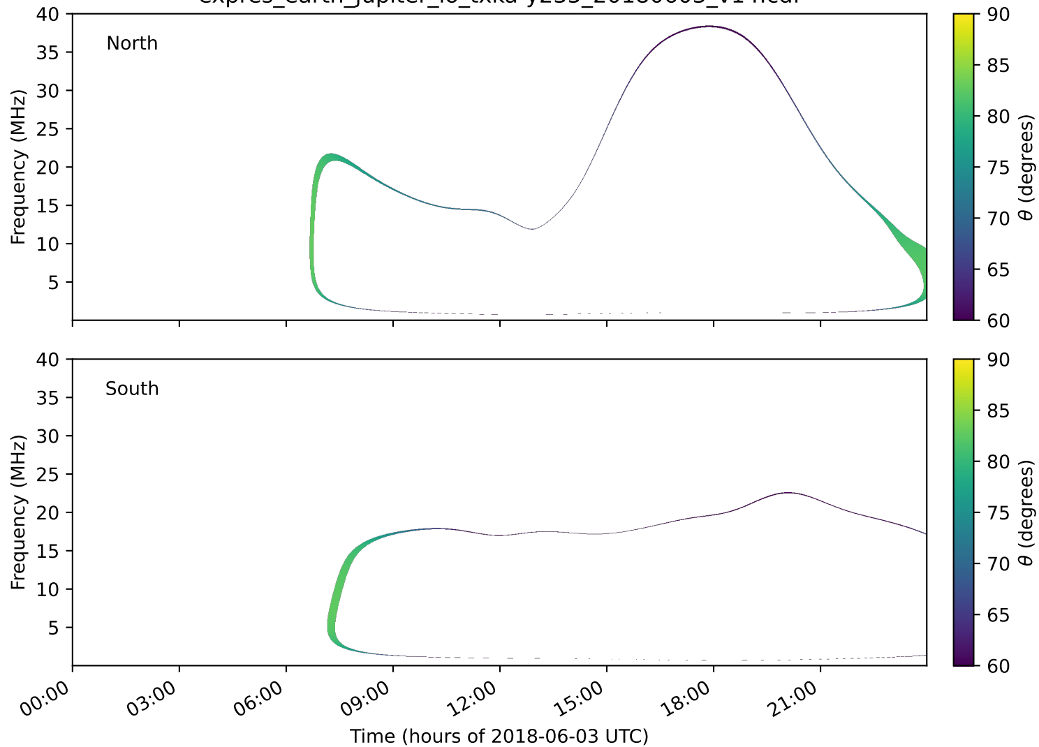
expres_earth_jupiter_io_txka-y235_20180603_v14.cdf
