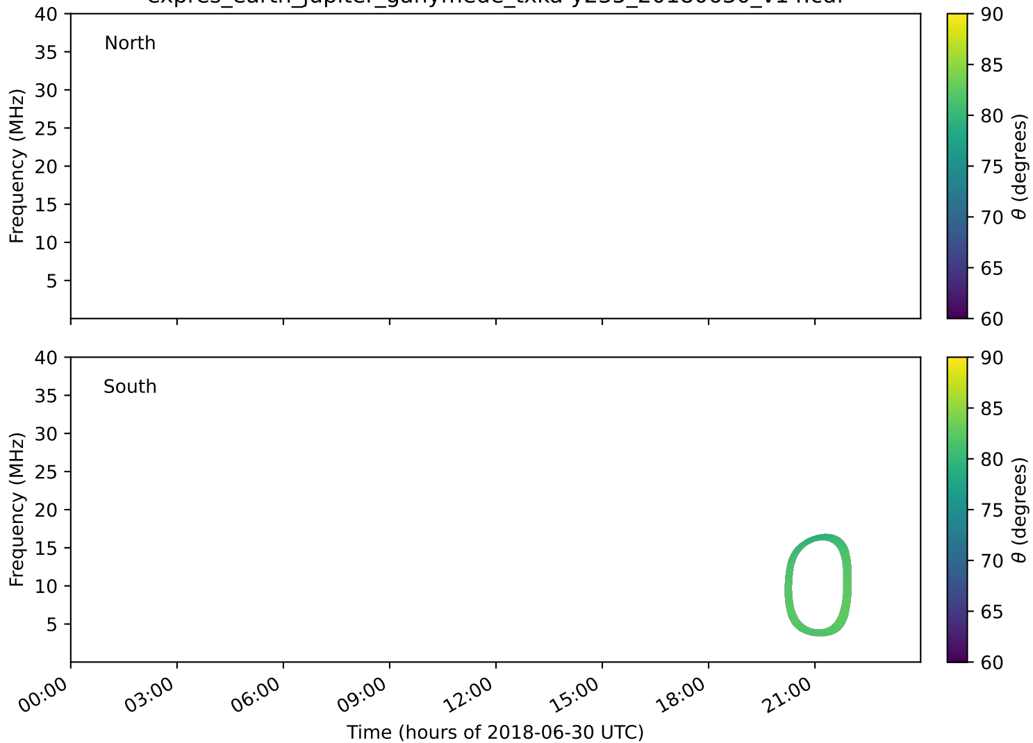
expres_earth_jupiter_ganymede_txka-y235_20180630_v14.cdf
